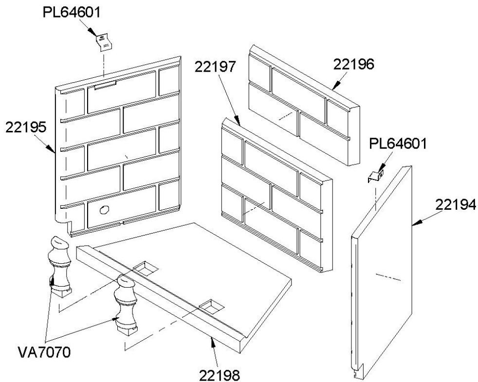
Figure 41: Replacing Antoinette refractory panels
